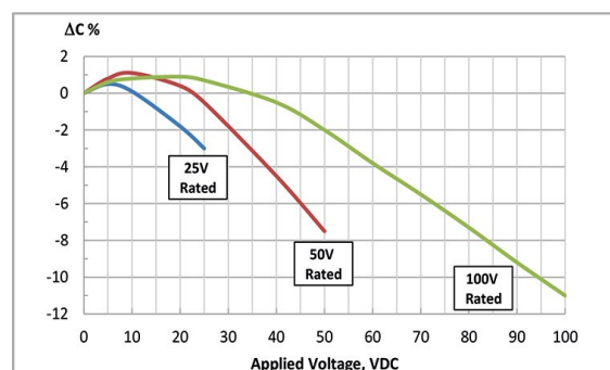
BX Voltage coefficient of capacitance
