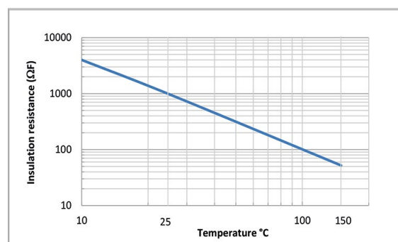
X7R and BX Insulation resistance vs temperature
